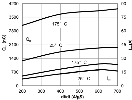
Fig 23: Diode Reverse Recovery Charge and Peak Current vs. di/dt ( V_{GE}=15V, V_{CE}=400V, I_F=60A )
