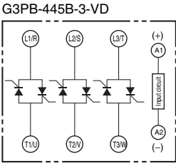
Terminal Arrangement/Internal Circuit Diagram
