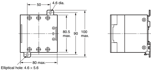
With Terminal Cover
