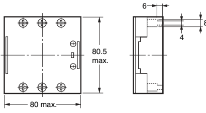
With Terminal Cover
