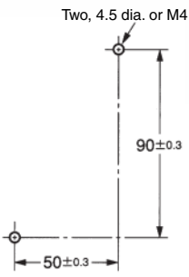
Mounting Holes
