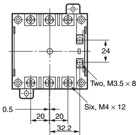
Mounting holes
