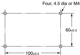
Mounting Holes
