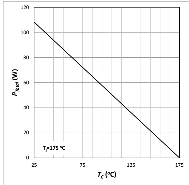
Fig. 4 Power Derating
