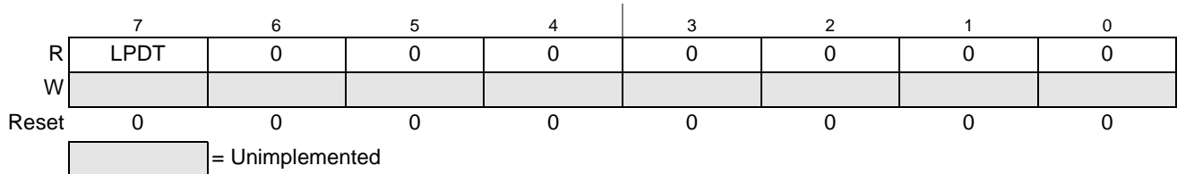
Figure 18-8. LIN Status Register (LPSR)
