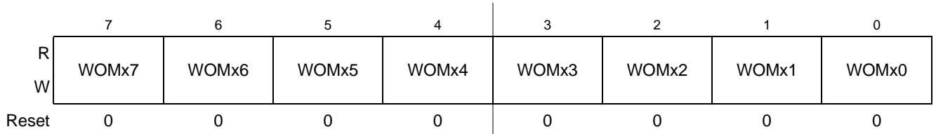
Figure 2-20. Wired-Or Mode Register
