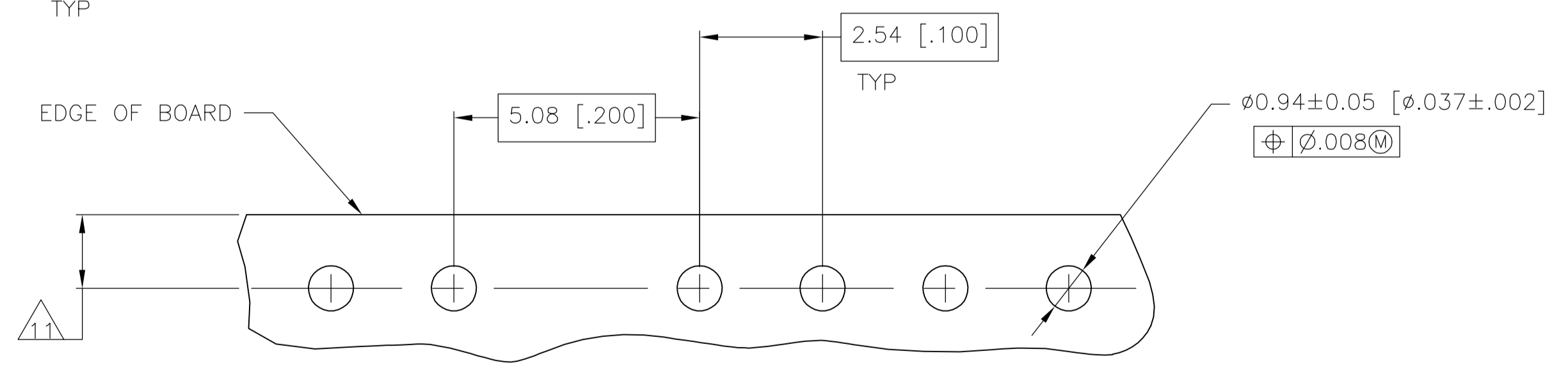
RECOMMENDED MOUNTING HOLE PATTERN FOR 1.60 [.063] THICK P.C. BOARD
