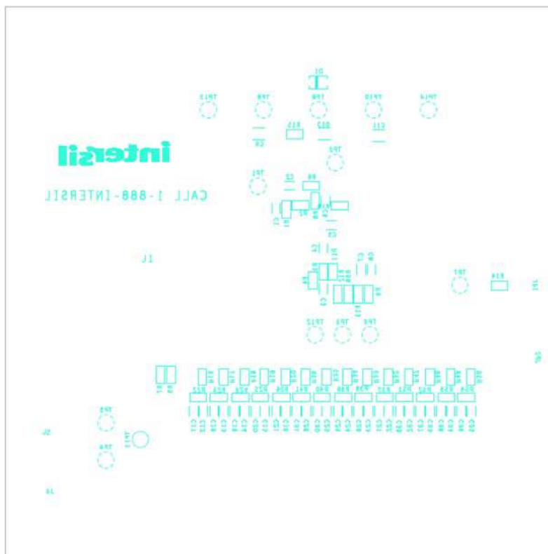
FIGURE 20. SILKSCREEN BOTTOM
