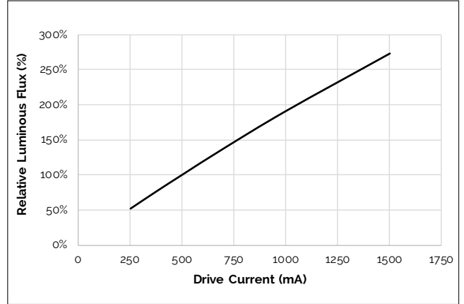
Figure 2: V15D Typical Relative Flux vs. Current
