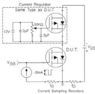
Fig 9b. Gate Charge Test Circuit
