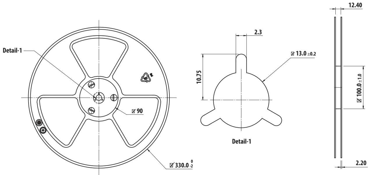
Figure 17 Reel Dimensions
