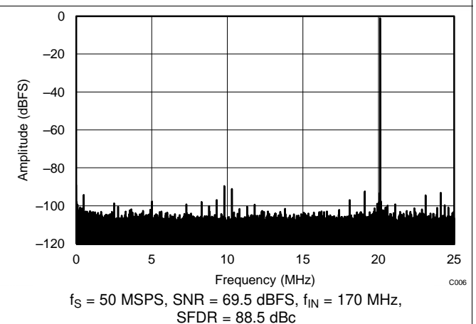
Figure 105. FFT for 170-MHz Input Signal (Dither Off)
