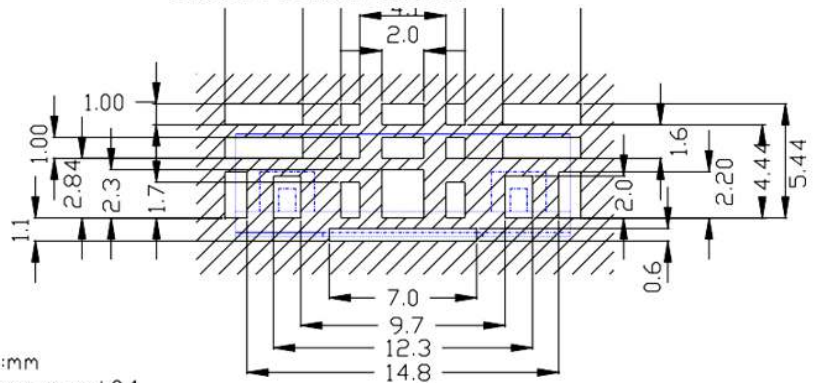
3-2-2 Solder Resist Pattern
