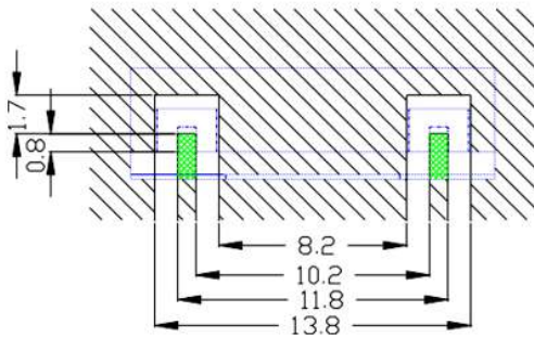
3-2-1 Conductive Material Pattern
