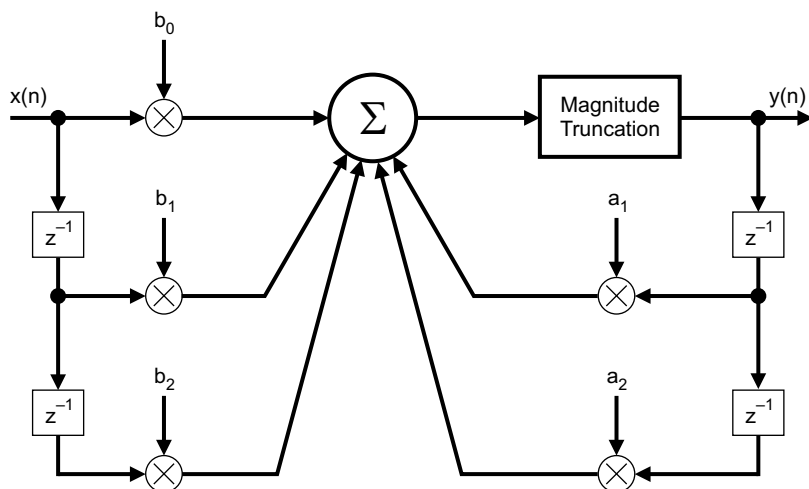
Figure 47. Biquad Filter
