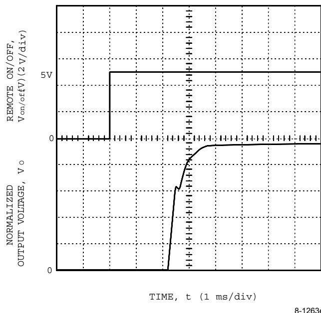
Figure 9. LUW025A, F Typical Output Voltage Start-Up when Signal Is Applied to Remote On/Off
