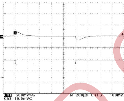
Figure 8. QMS14DG, Load Response (typ)
