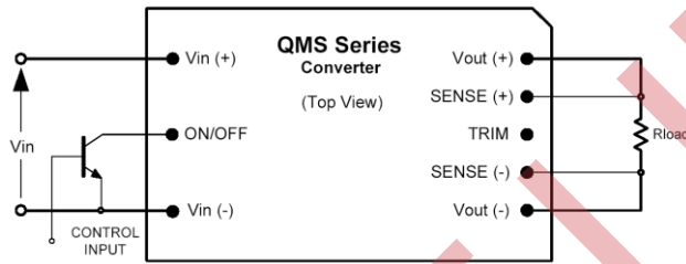
Figure 30. On/Off Control
