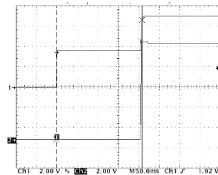
Figure 5. QMS07DH, Turn-On via On/Off Ctrl (typ)
