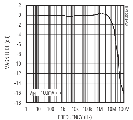
SMALL-SIGNAL RESPONSE
