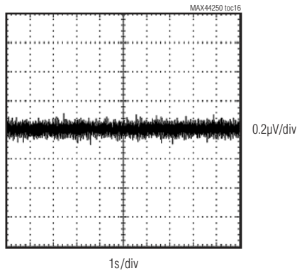
INPUT VOLTAGE 0.1Hz TO 10Hz NOISE
