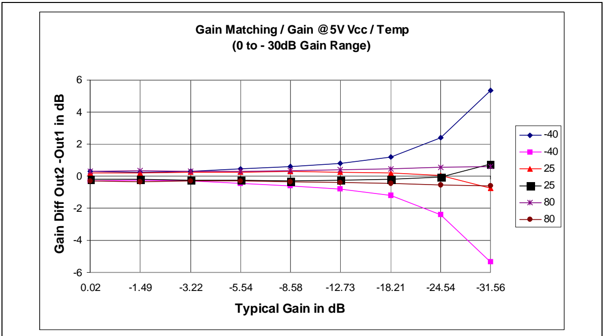
Figure 19 - Typical Gain Matching / AGC @ 5V Vcc / Temp
