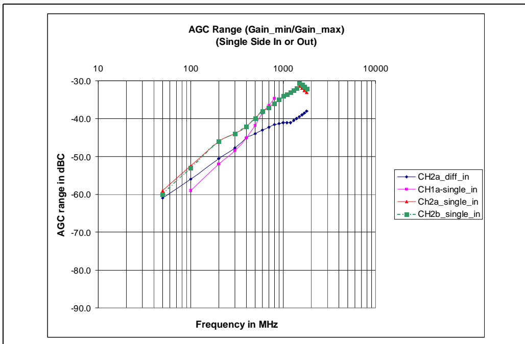
Figure 15 - Typical AGC Range / Frequency (Single Ended output)
