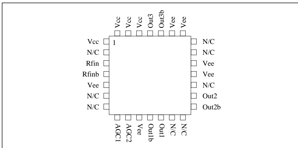
Figure 2 - Pin Diagram
