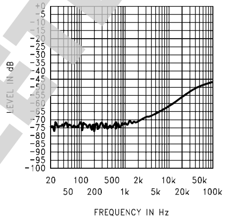
Input Floating
