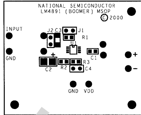
Silk Screen
