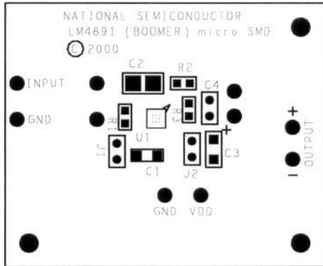
Silk Screen
