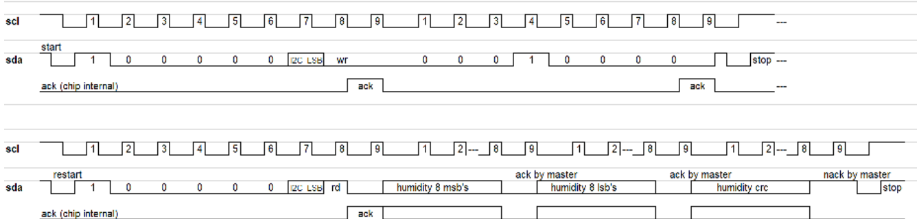
Figure 7 Read RH Command
