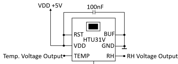
Figure 4 HTU31V Typical Application Circuit
