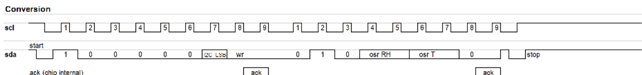
Figure 5 Conversion Command
