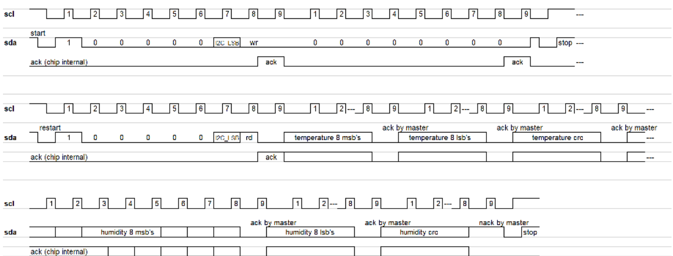
Figure 6 Read T&RH command
