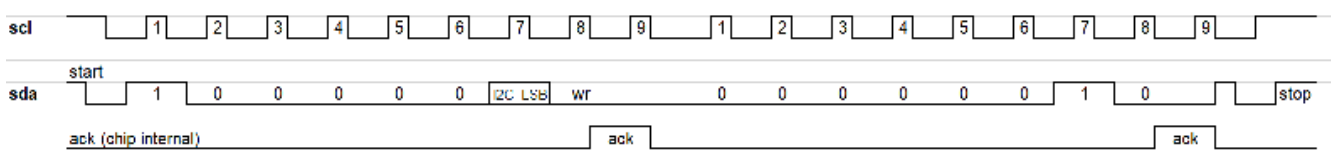
Figure 10 Heater off Command
