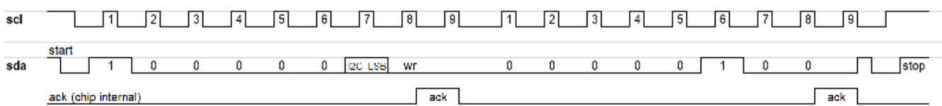
Figure 9 Heater on Command
