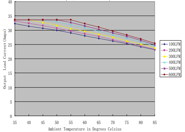
Figure 13. Temperature derating, current, longitudinal airflow Vin to Vout 48V Input, 10" X 10" test pcb
