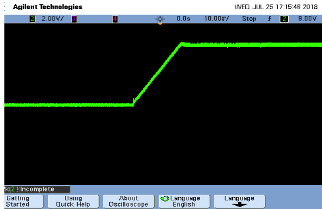
Figure 22. Output Pre-bias start-up Vin=48V, Iout = 0A, Cloud = 47µF, Ta = 25°C, Pre-bias Voltage = 6V
