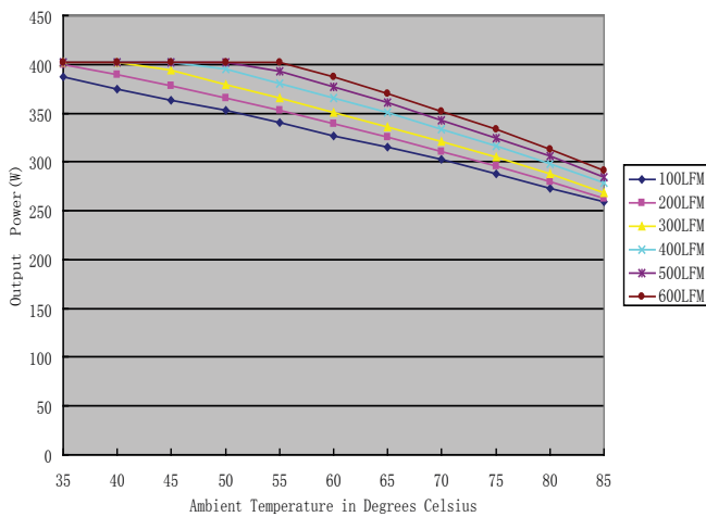
Figure 14. Temperature derating, power, longitudinal airflow Vin to Vout 75V Input, 10" X 10" test pcb
