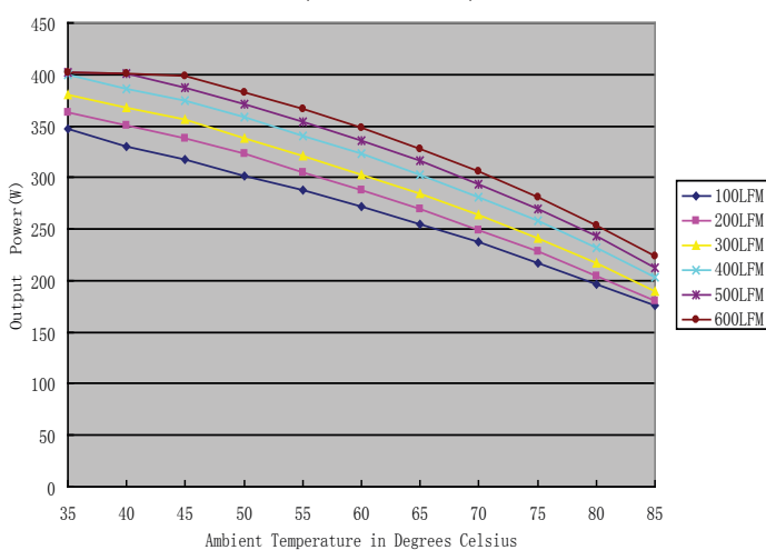
Figure 14. Temperature derating, power, longitudinal airflow Vin to Vout 75V Input, 10" X 10" test pcb
