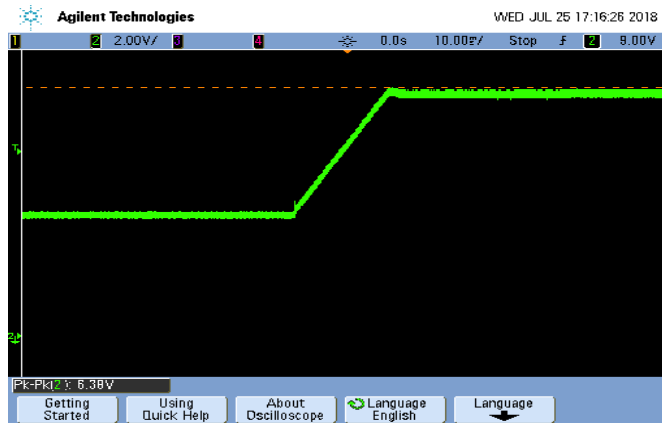
Figure 25 Output Pre-bias start-up Vin=48V, Iout = 0A, Cloud = 10000µF, Ta = 25°C, Pre-bias Voltage = 9.6V
