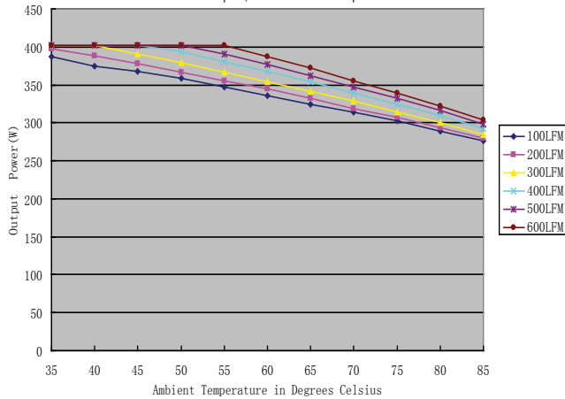
Figure 12. Temperature derating, power, longitudinal airflow Vin to Vout 48V Input, 10" X 10" test pcb
