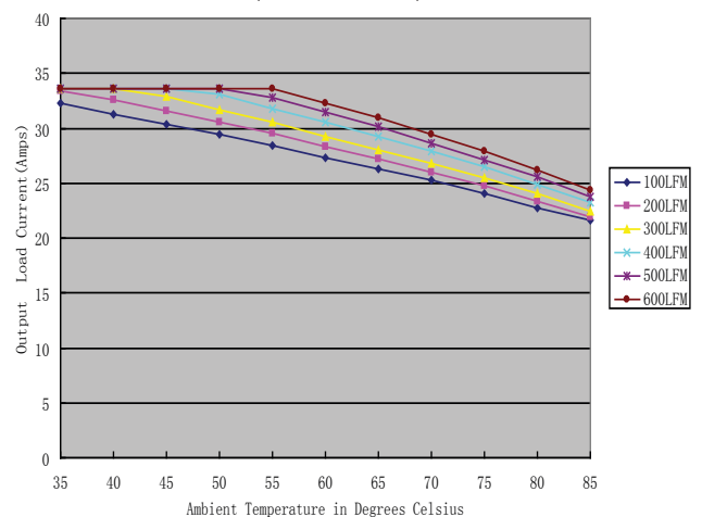
Figure 15. Temperature derating, current, longitudinal airflow Vin to Vout 75V Input, 10" X 10" test pcb
