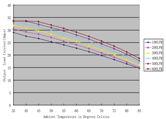
Figure 15. Temperature derating, current, longitudinal airflow Vin to Vout 75V Input, 10" X 10" test pcb
