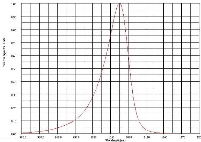
SPECTRAL OUTPUT
