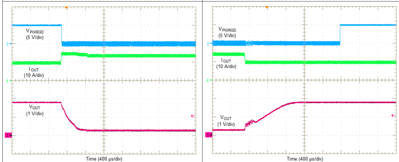
Figure 35. Overcurrent Limiting (Cycle-by-Cycle)
