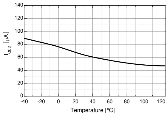
Figure 10. Quiescent V_{DD} Supply Current vs. Temperature
