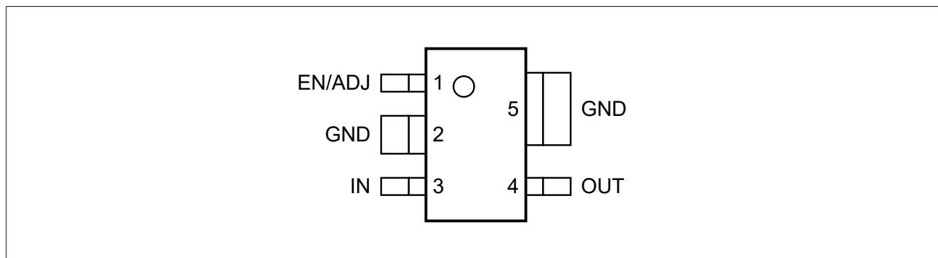
Figure 2 Pin configuration
