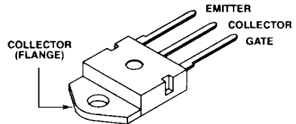
HGTH-TYPES JEDEC TO-218AC
