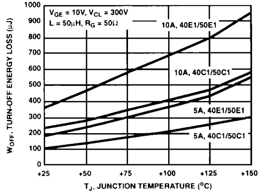
FIGURE 14. TYPICAL CLAMPED INDUCTIVE TURN-OFF SWITCHING LOSS/WAVEFORM
