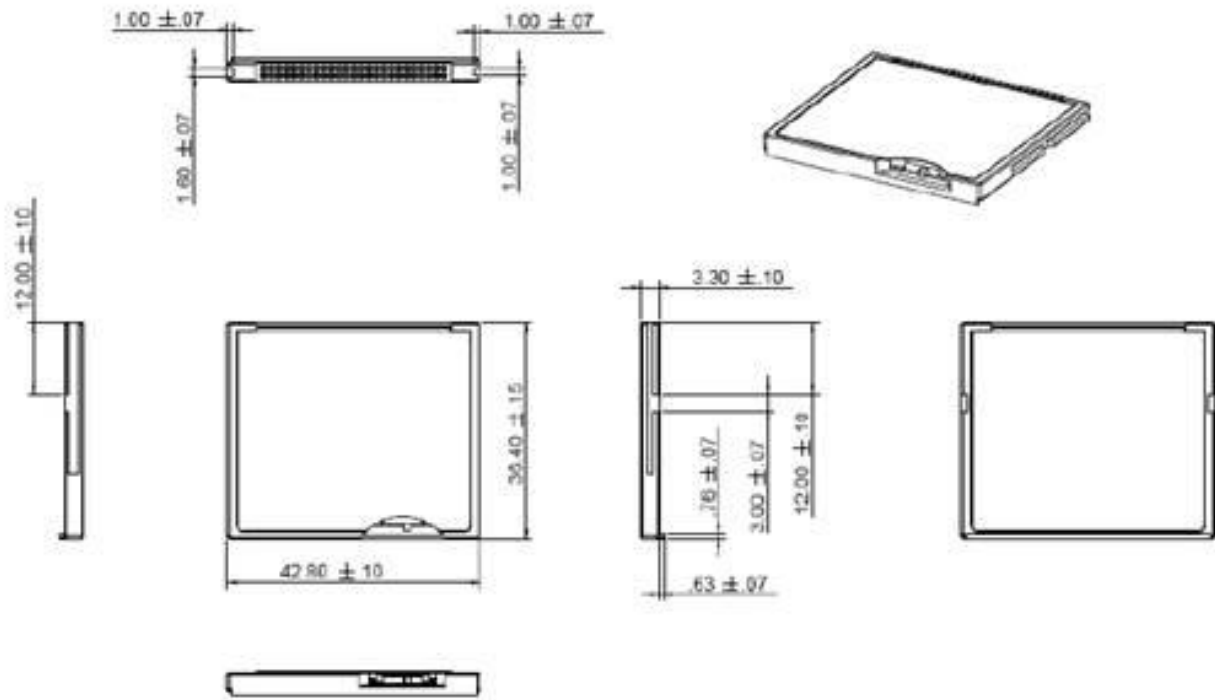
Figure 7-2 Physical Dimensions
