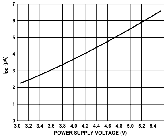
Figure 10. Shutdown I_{DD} vs. Power Supply
