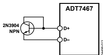
Figure 25. Measuring Temperature Using an NPN Transistor
