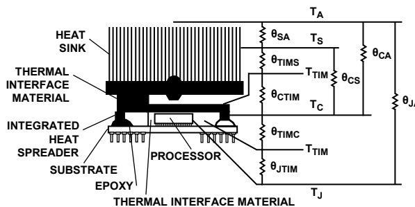
Figure 51. Thermal Model
