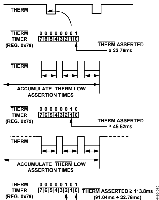
Figure 31. Understanding the \overline{\text{THERM}} Timer
