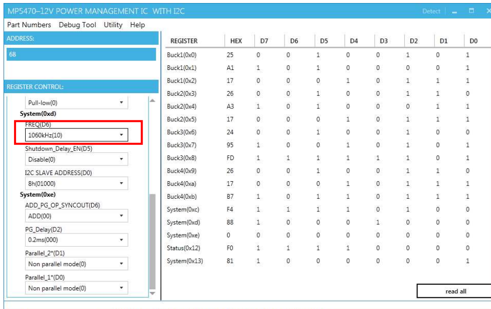
Figure 12: Parameters Modification via I2C Interface
