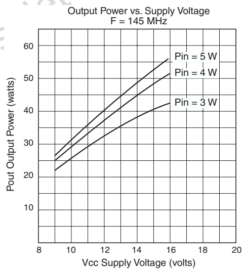
Figure 6. Power Output vs Supply Voltage (145 MHz)
