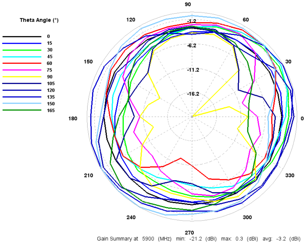
Figure 11: Total gain pattern
