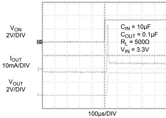
Figure 15. t dON Response
