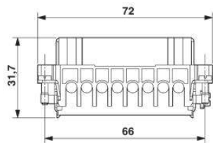
Female insert
