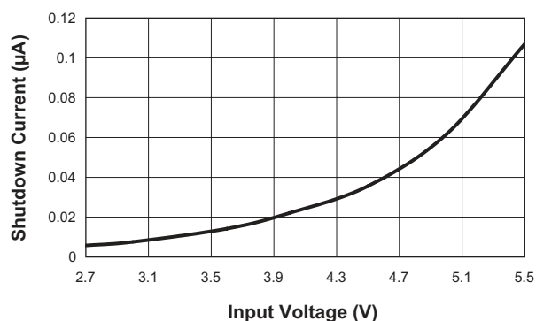
Shutdown Current vs. Input Voltage (EN/SET = FLEN = 0V)
