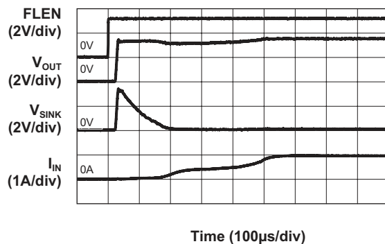
Flash Mode Turn On (500mA/ch)
