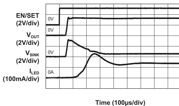
Movie Mode Turn On (68.5mA/ch)
