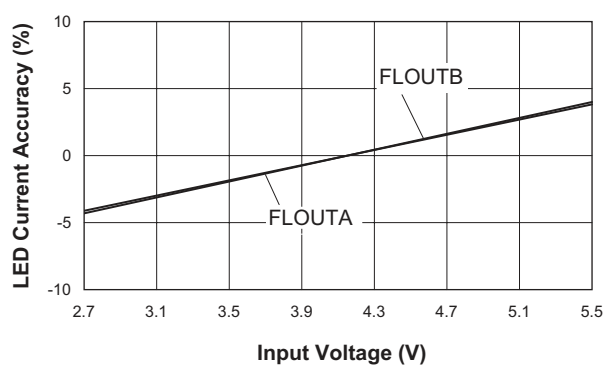
Movie Mode LED Current Accuracy vs. Input Voltage (68.5mA/Ch)
