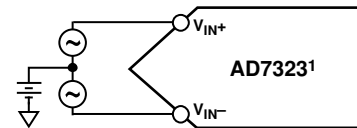
Figure 34. True Differential Inputs
