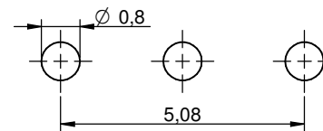
P.C.B. MOUNTING PLAN
