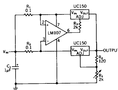
6A Regulator
