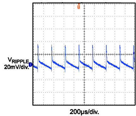
Output Ripple V_{IN} = 115V_{AC} , No Load
