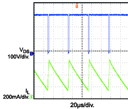
Normal Operation V_{IN} = 230V_{AC} , Full Load
