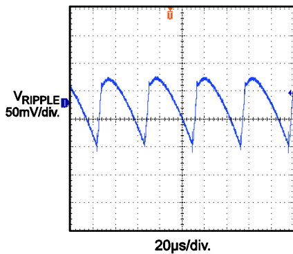
Output Ripple V_{IN} = 115V_{AC} , Full Load
