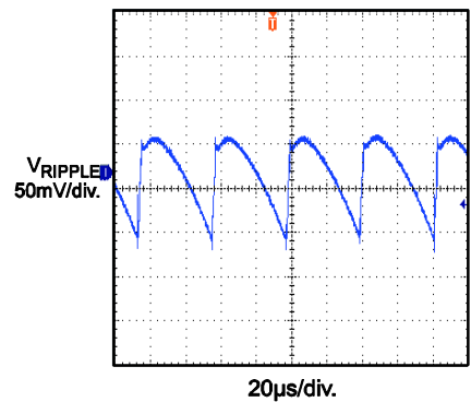
Output Ripple V_{IN} = 230V_{AC} , Full Load
