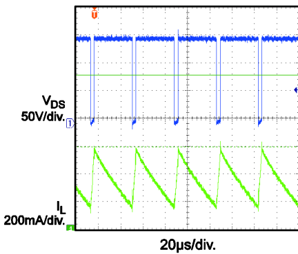
Normal Operation V_{IN} = 115V_{AC} , Full Load
