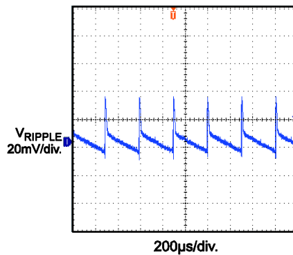
Output Ripple V_{IN} = 230V_{AC} , No Load
