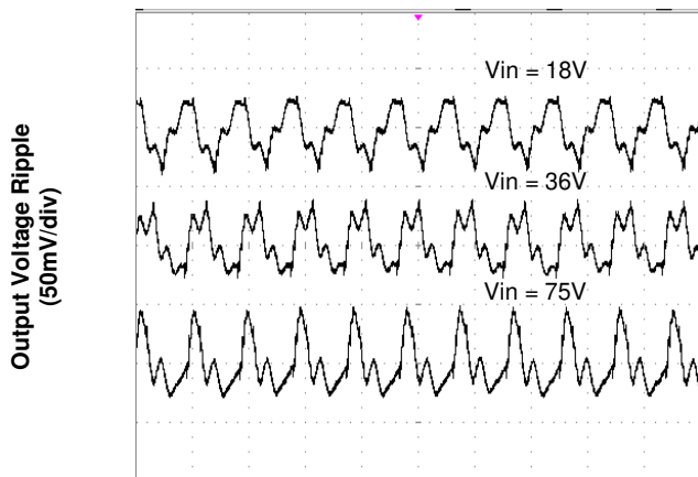
Figure 5. Output Ripple Voltage at Full Load
