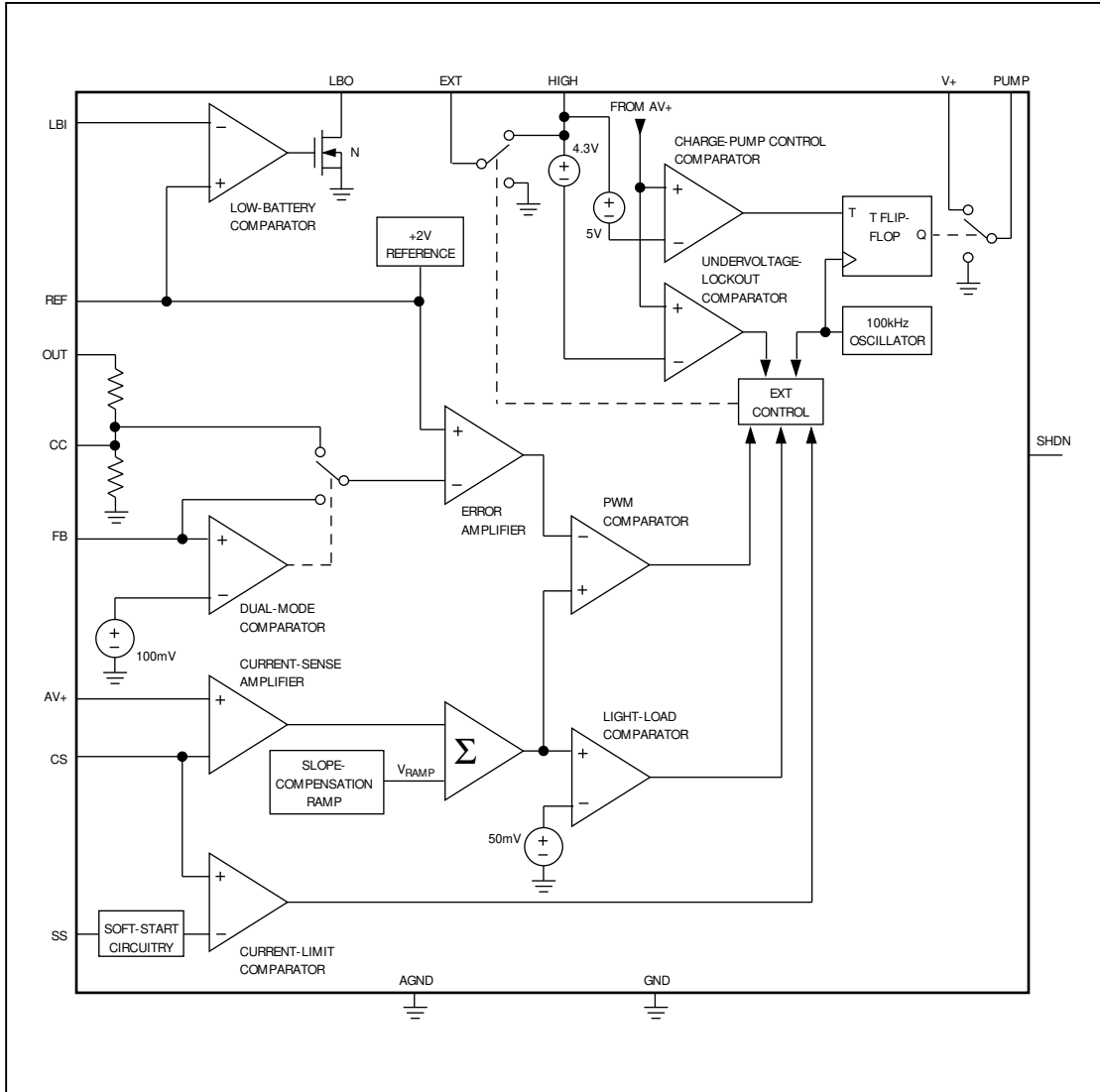
Figure 2. Block Diagram
