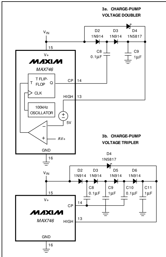
Figure 3. Charge-Pump Configurations
