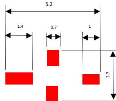
PCB Footprint
