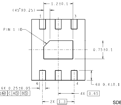
6-Pin LLP NS Package Number SDB06A
