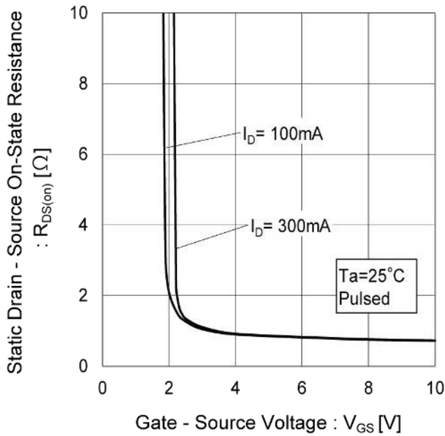
Fig.7 Static Drain - Source On - State Resistance vs. Gate Source Voltage
