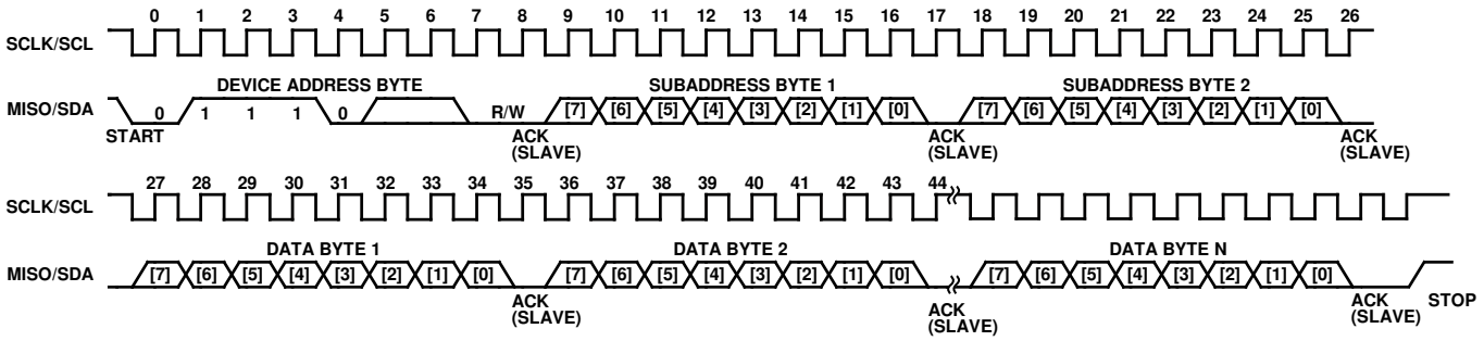
Figure 26. I 2 C Slave Burst Mode Write Operation (N Bytes)
