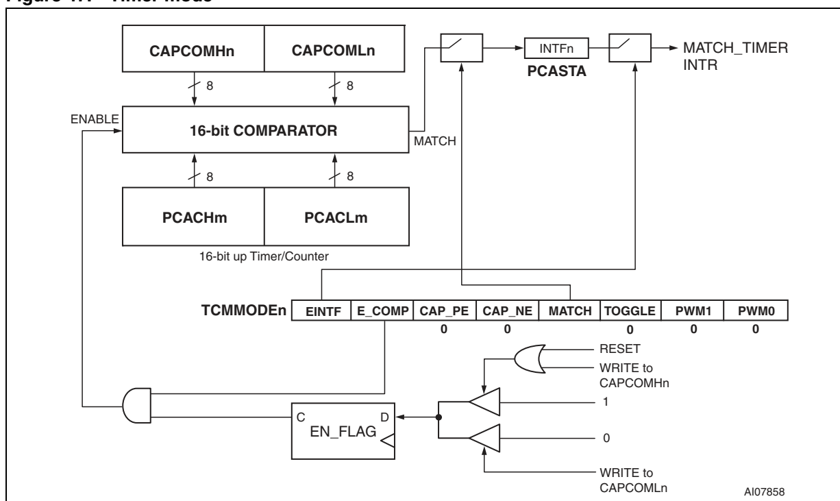
Figure 47. Timer mode
