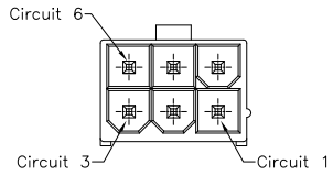
6PIN
