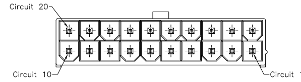
20PIN
