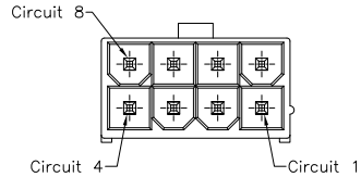
8PIN
