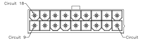
18PIN
