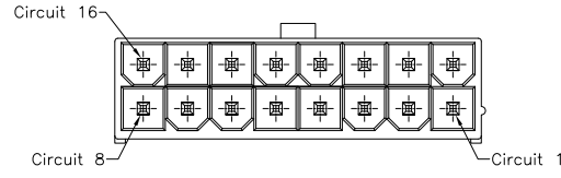
16PIN
