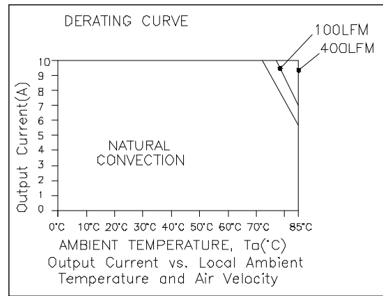
Figure 33. Vo = 1.8 V
