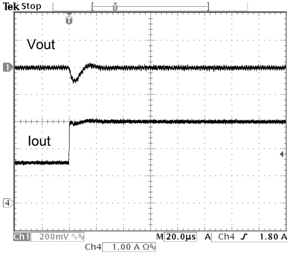
Fig.14: Output voltage response to step load change at 5A/us from 50% to 100% (12Vin, 1.8Vout)
