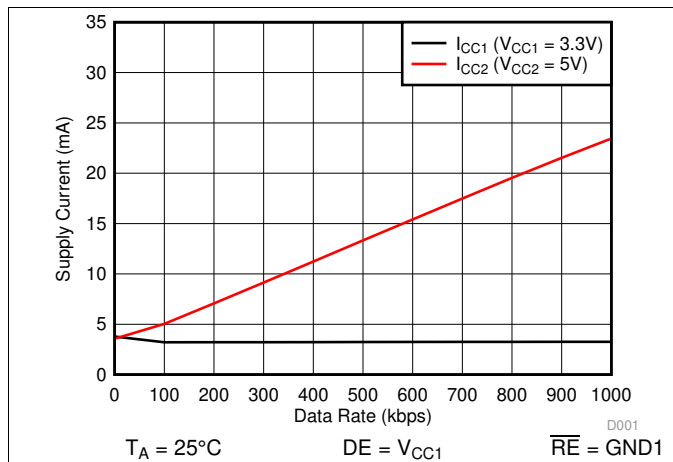
Figure 3. Supply Current Vs Data Rate- No Load
