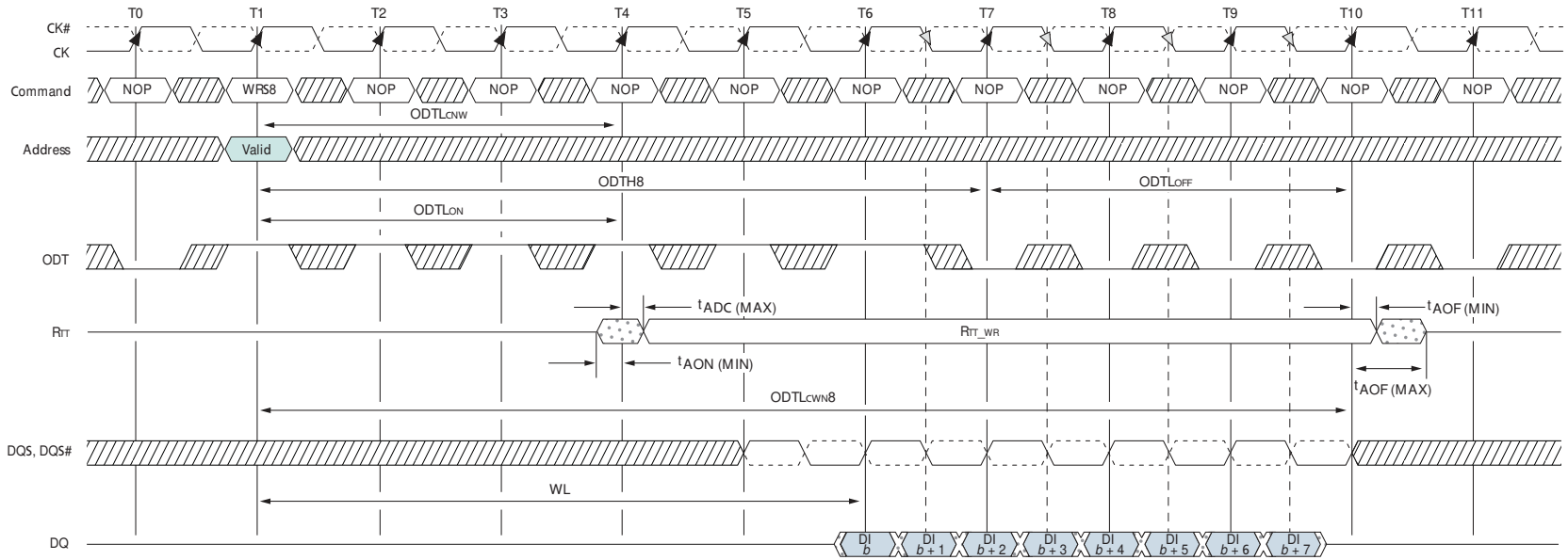
Figure 113: Dynamic ODT: ODT Pin Asserted Together with WRITE Command for 6 Clock Cycles, BL8
