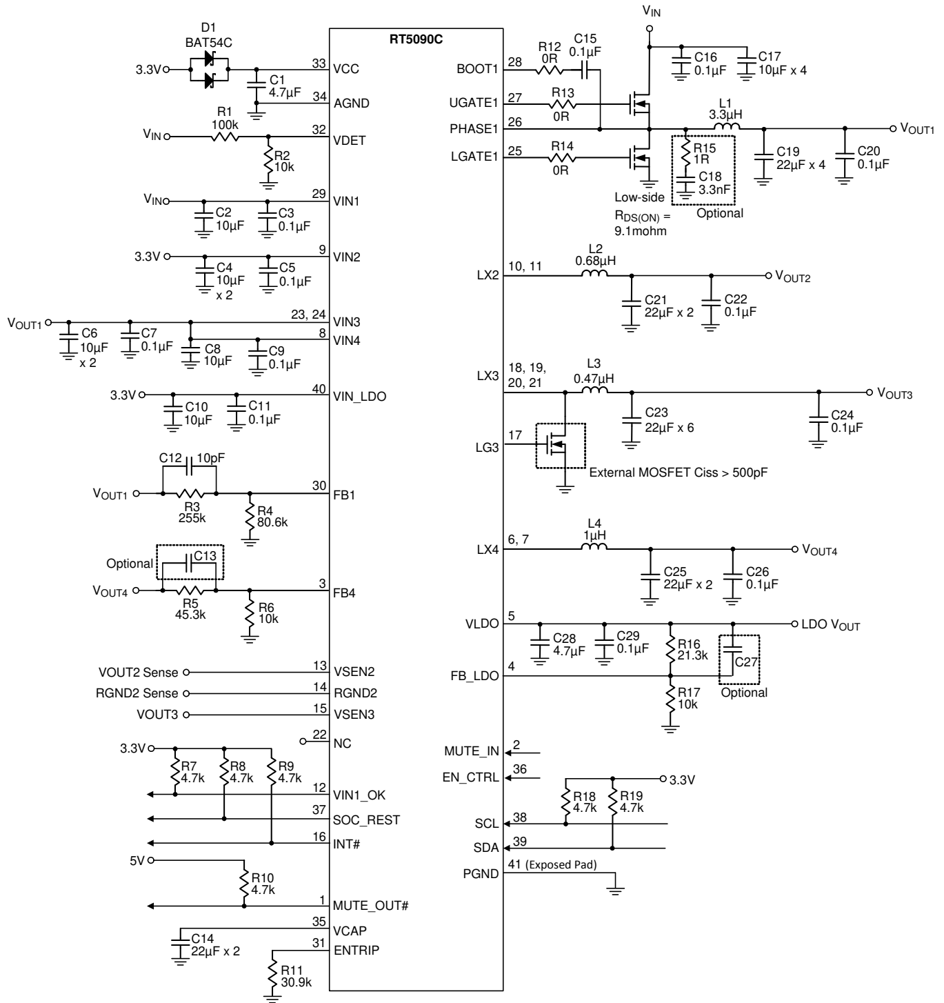
Figure 2. For 12V + 3.3V Standby System
