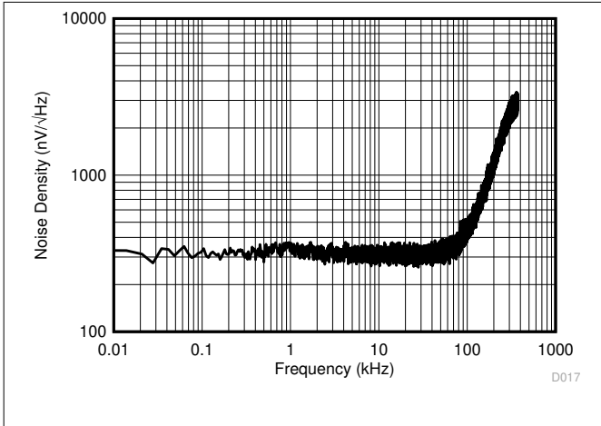
Figure 6-29. Input-Referred Noise Density vs Frequency
